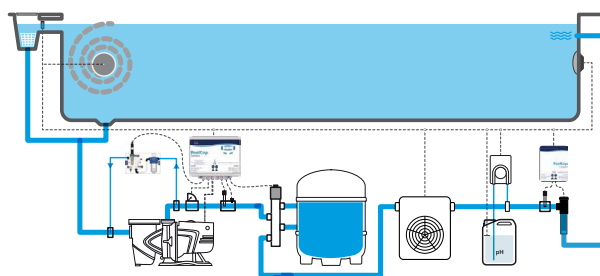
TYPICAL ELECTROLYSIS INSTALLATION
