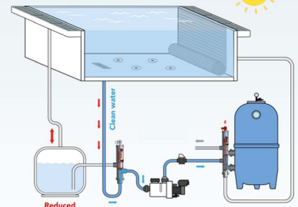
BACKWASHES DIRECTLY FROM THE POOL
