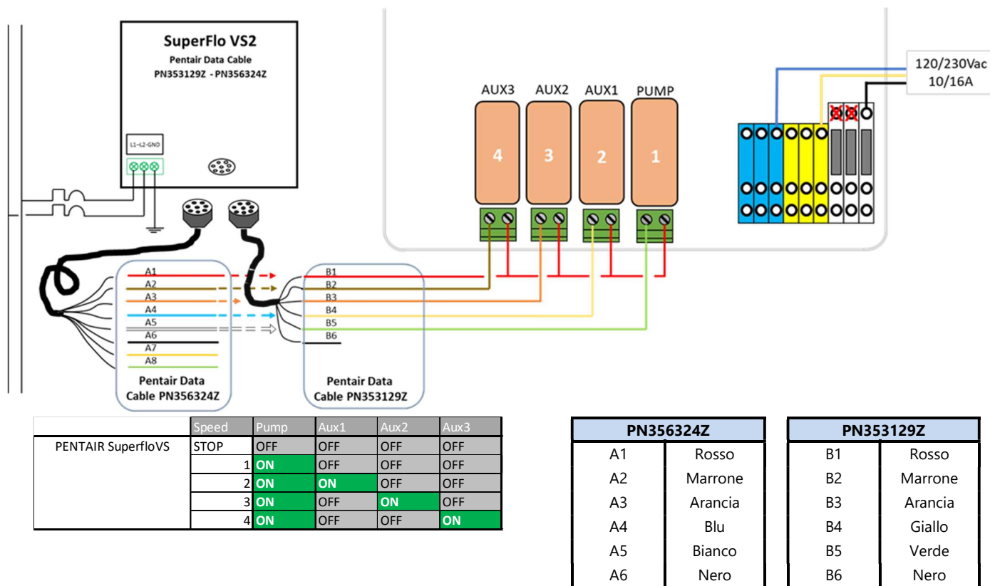
Figura 21 - Pentair SuperFlo VS/VS2
