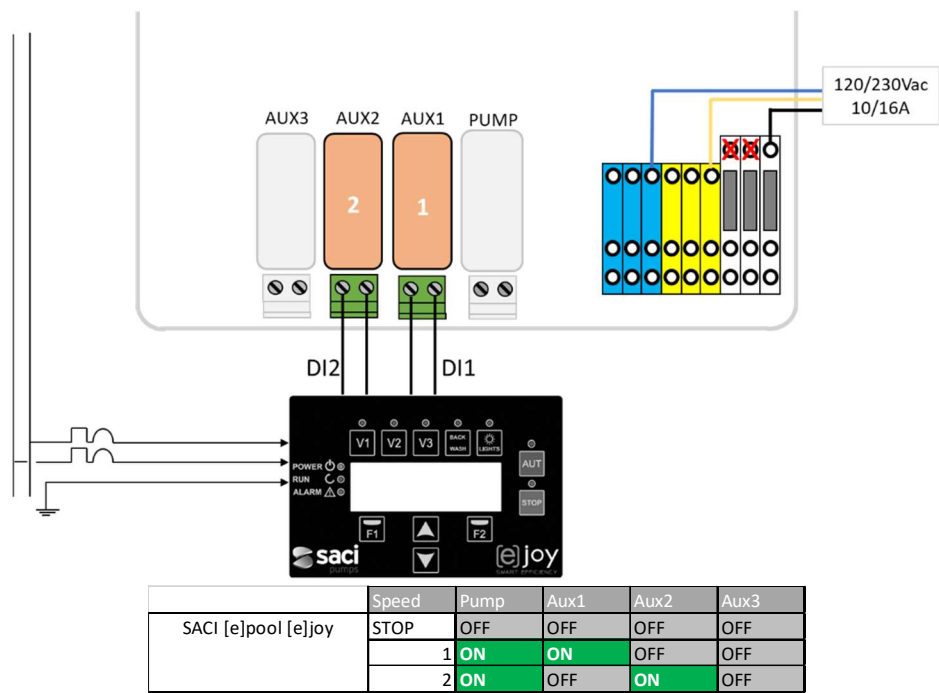
Figura 32 - SACI [e]pool, [e]joy
