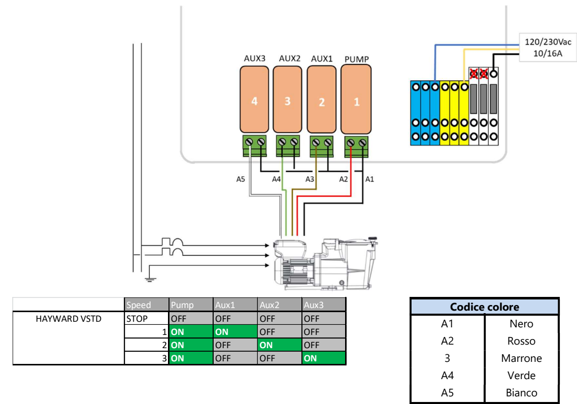
Figura 23 - Hayward game VSTD
