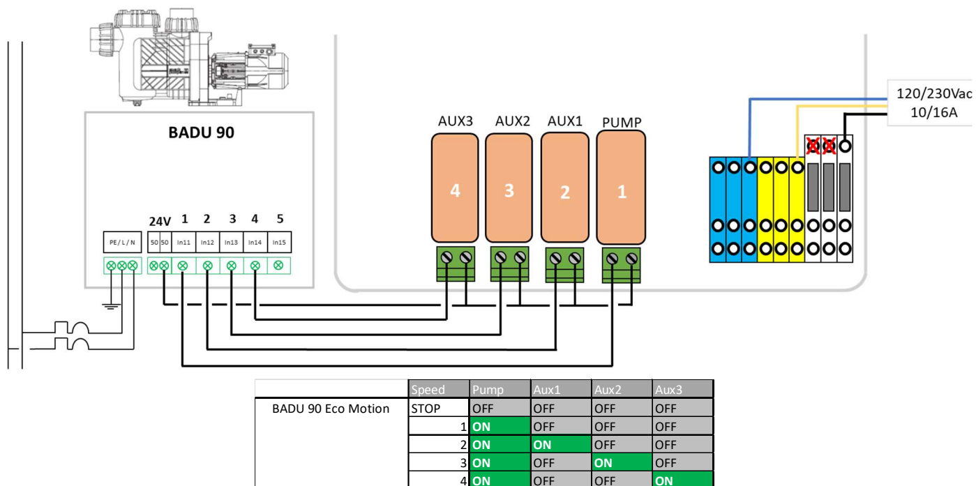
Figura 25 - Speck Badu Eco-Motion
